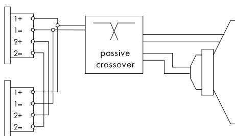
Connector wiring
