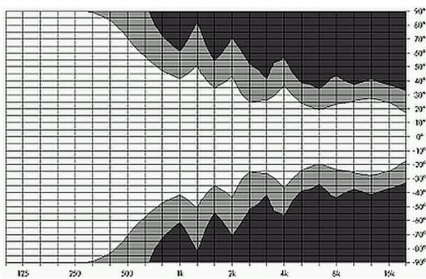
Isobar diagram E12-D horizontal, horizontal setup with the horn rotated
