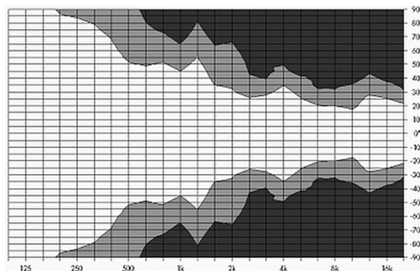
Isobar diagram E12 vertical, standard setup
