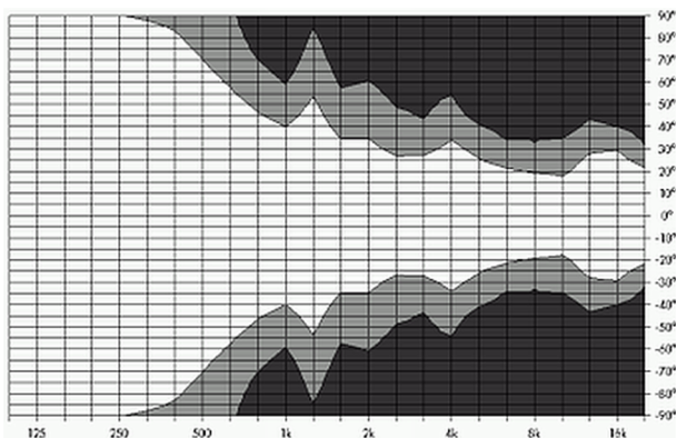
Isobar diagram E12 horizontal, horizontal setup with the horn rotated
