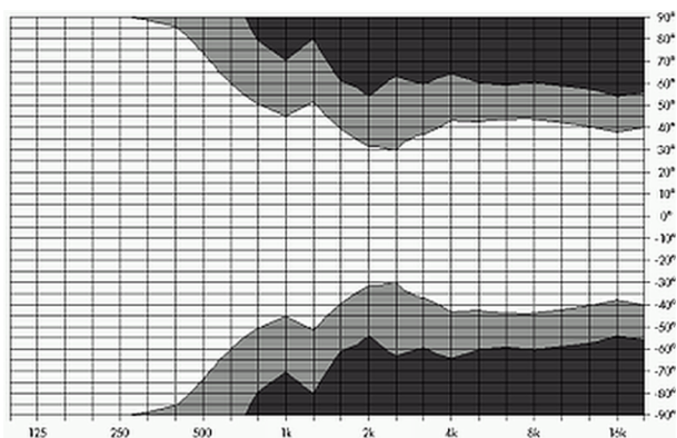
Isobar diagram E12 horizontal, standard setup
