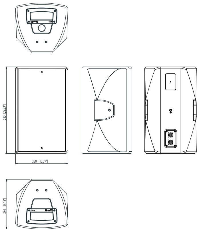
E12/E12-D cabinet dimensions in mm [inch]
