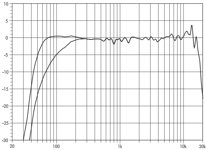
E12 frequency response, standard and CUT modes.
