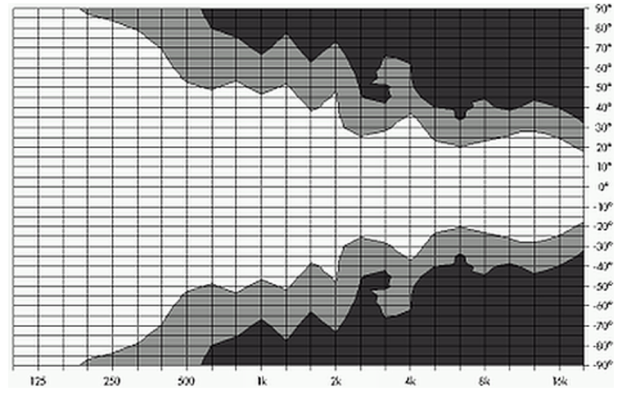
Isobar diagram E12-D vertical, standard setup
