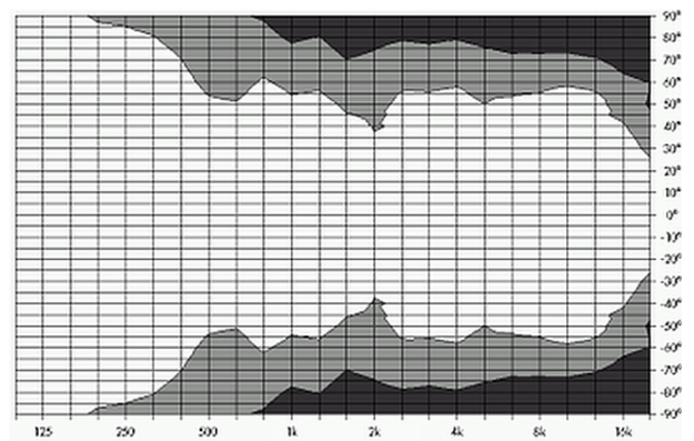
Isobar diagram E12-D vertical, horizontal setup with the horn rotated
