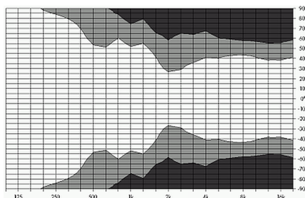
Isobar diagram E12 vertical, horizontal setup with the horn rotated
