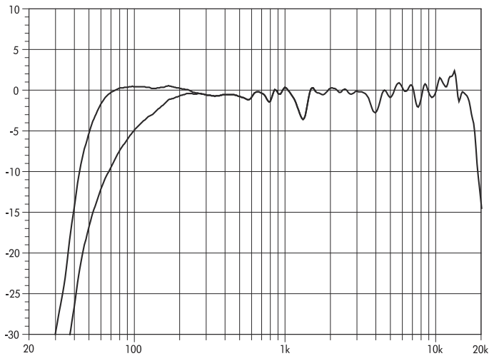
E12-D frequency response, standard and CUT modes.
