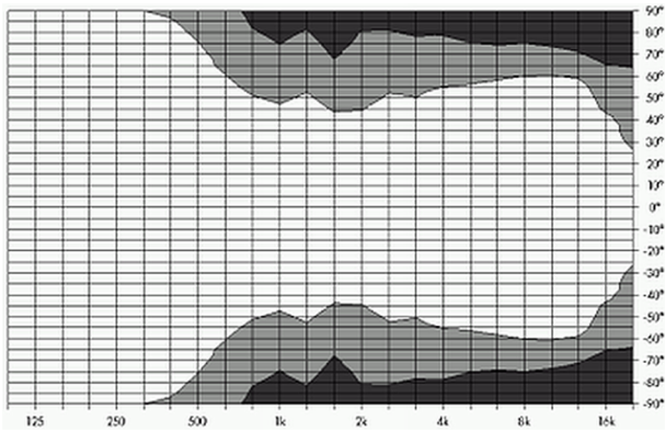
Isobar diagram E12-D horizontal, standard setup
